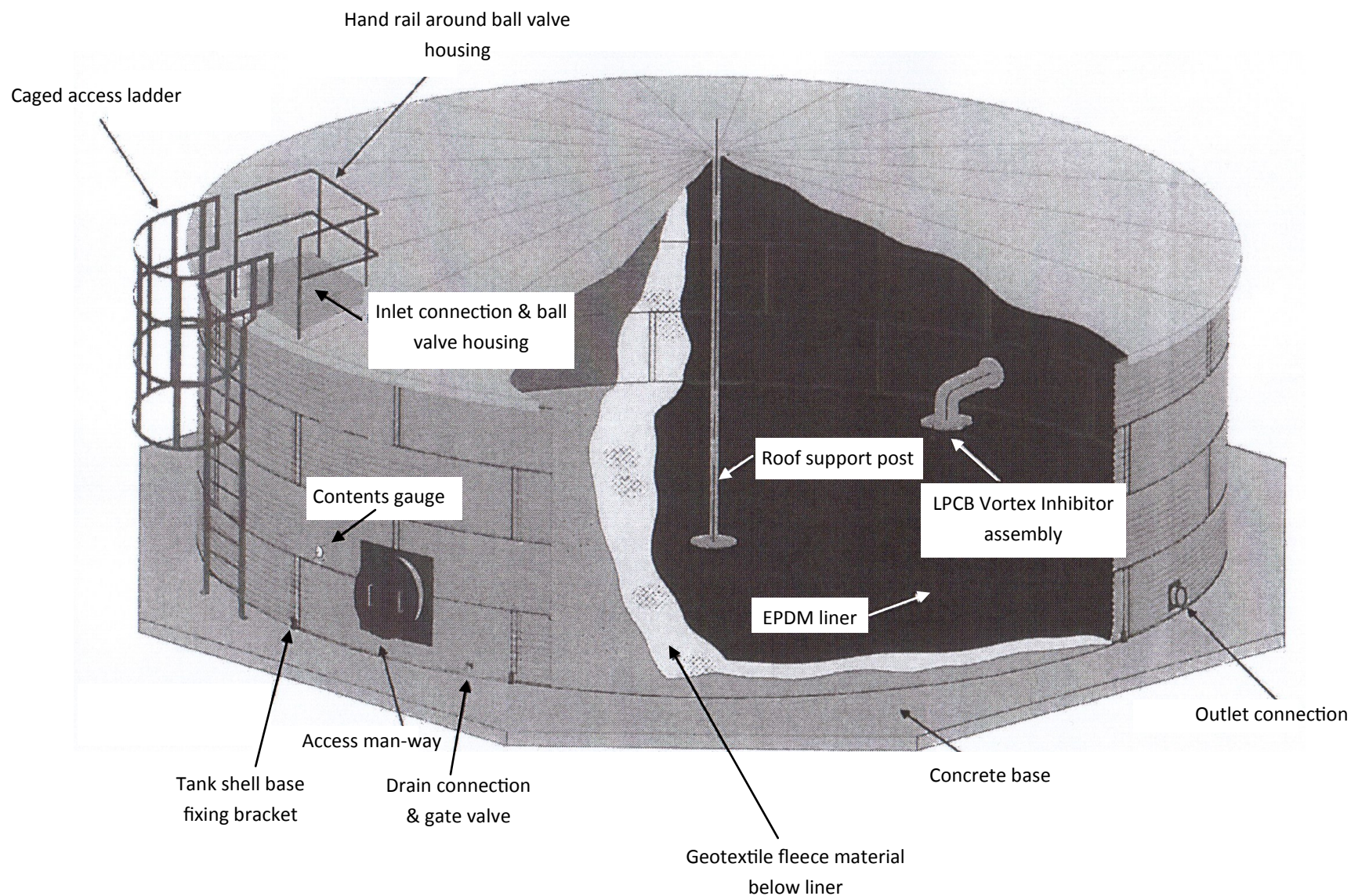
Typical LPCB Approved Fire Tank Drawing
